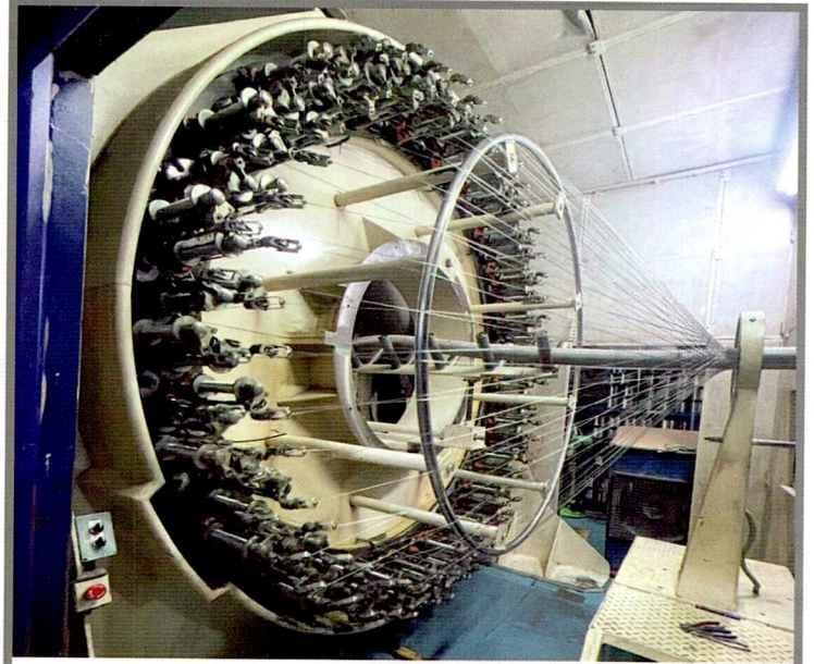
BRAID MANUFACTURING MACHINE
